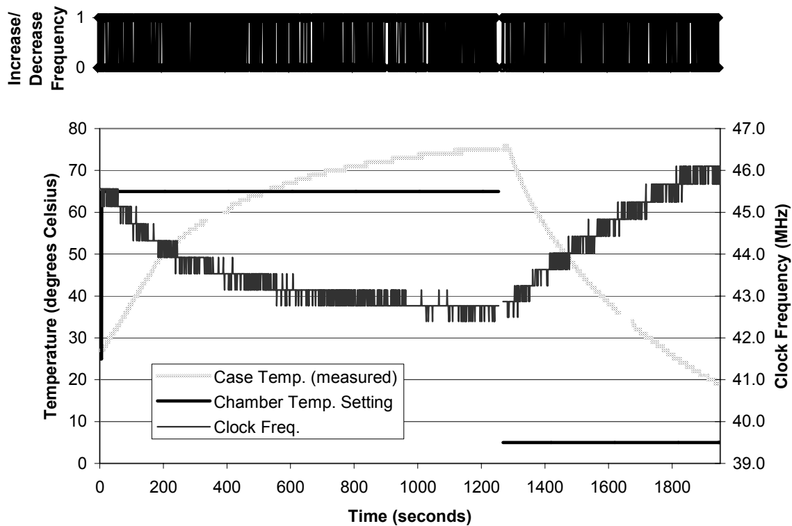
Fig. 10. Experiment 3: TEAtime rapid temperature change response. Each datum is a run sample taken every second; the CPU always runs, however.
