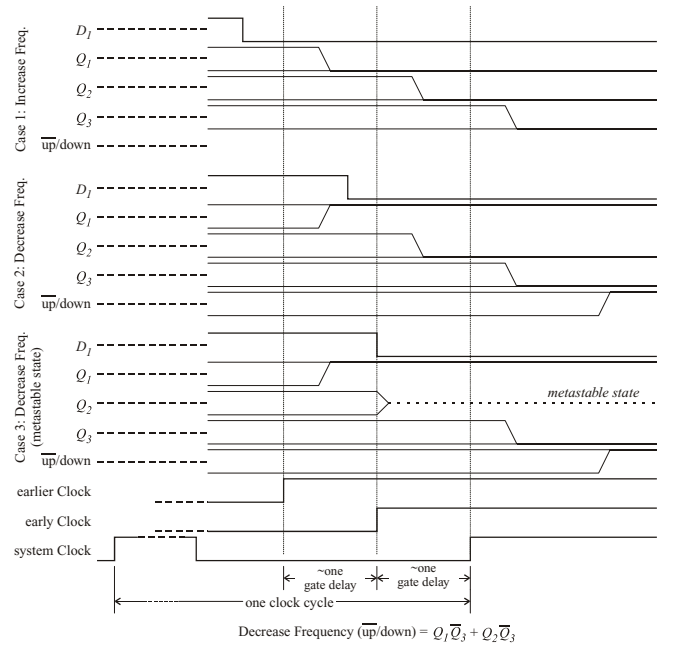
Fig. 4. Timing Checker / TEAtime detailed timing.
