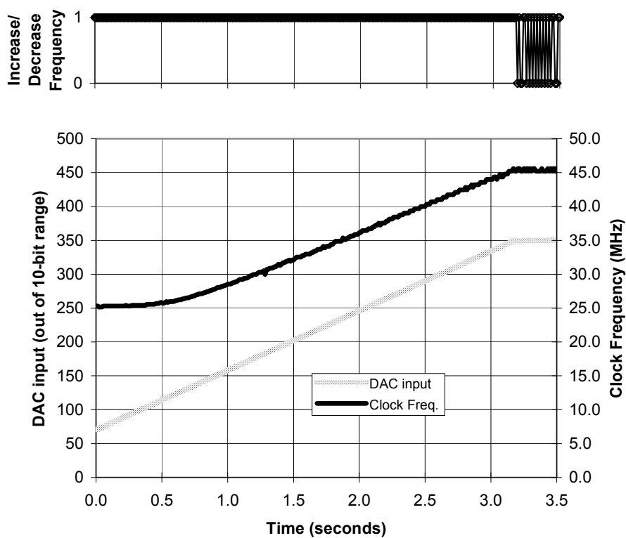
Fig. 7. Experiment 1, part A: TEAtime automatically rises to a high frequency and then stabilizes at that point.
