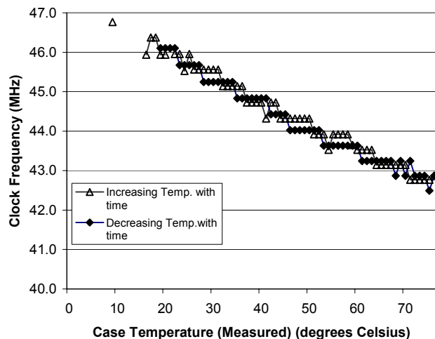
Fig. 11. System Clock Frequency vs. Case Temperature. Only one datum per degree C. is plotted.
