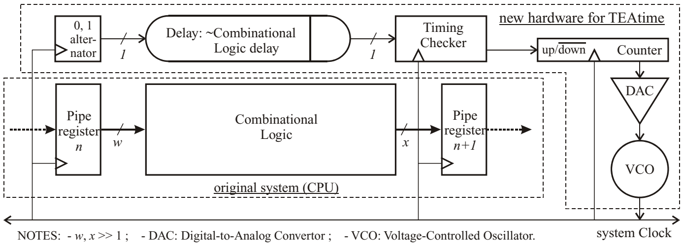
Fig. 1. Timing Error Avoidance (TEAtime) block diagram
