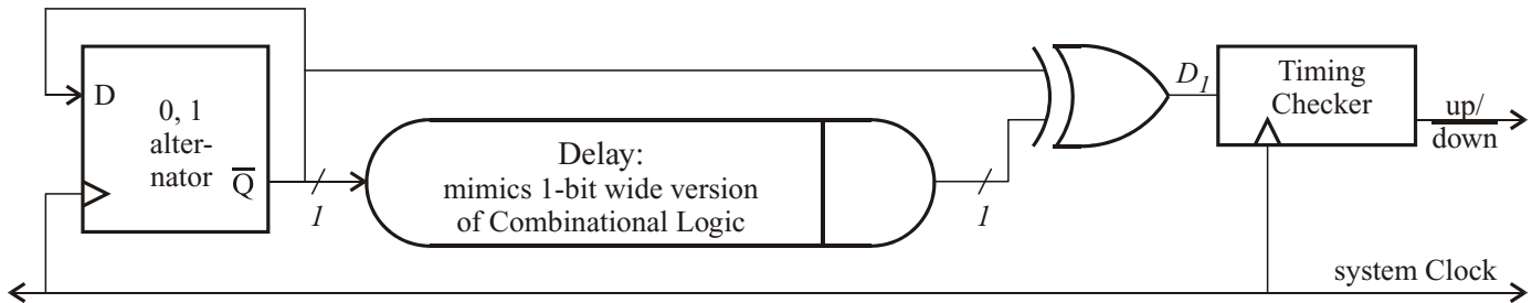
Fig. 2. Details of the main components of TEAtime circuitry.
