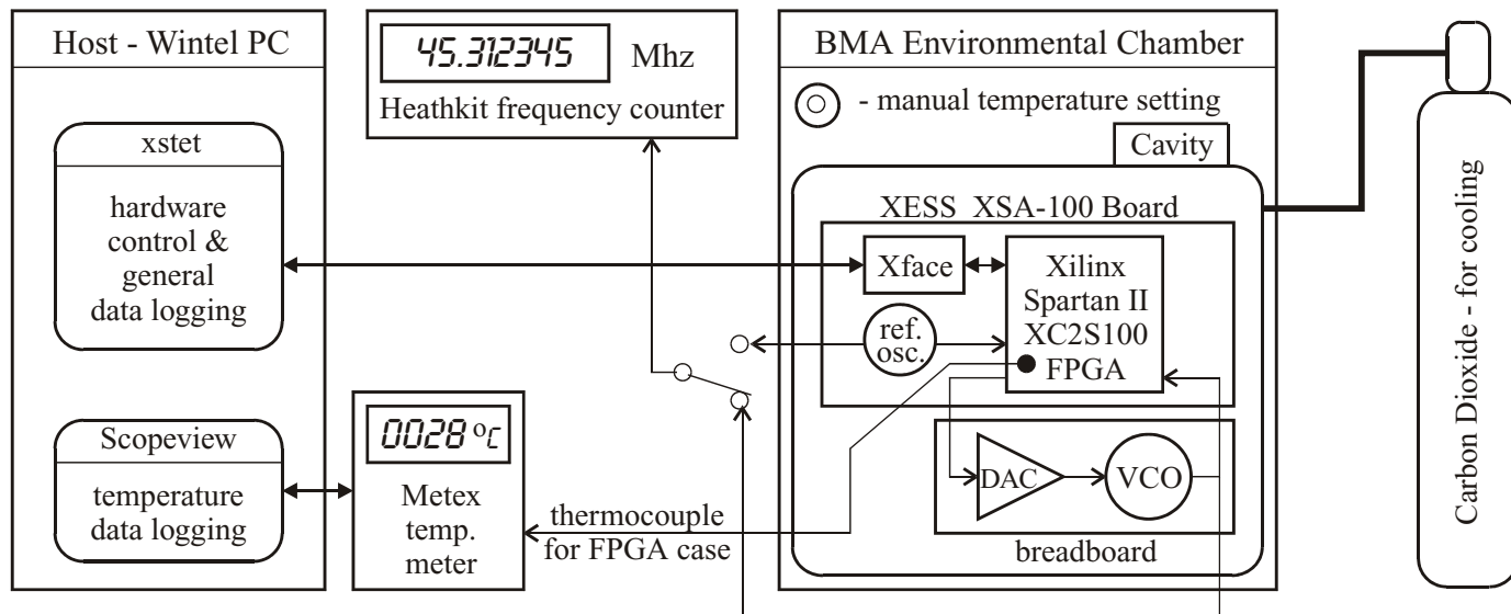
Fig. 5. TEAtime evaluation experimental setup.
