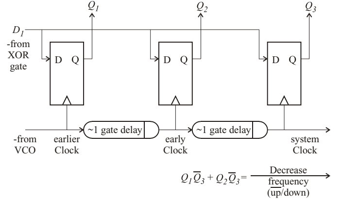
Fig. 3. Timing Checker detailed design.
