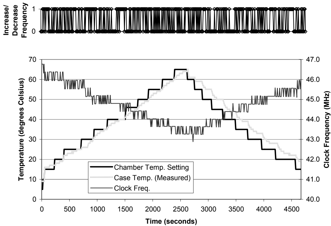
Fig. 9. Experiment 2: TEAtime gradual temperature change response. Each datum is a run sample taken every 10 seconds; the CPU always runs, however.
