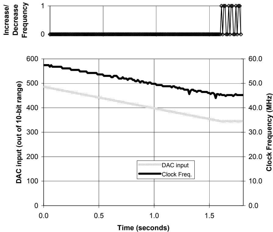
Fig. 8. Experiment 1, part B: Decreasing-frequency stabilization.
