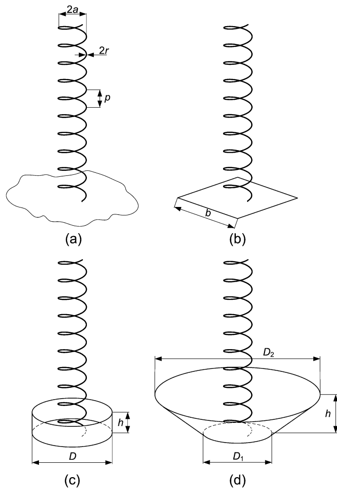
Fig. 1. Helical antenna above (a) infinite ground plane, (b) square conductor, (c) cylindrical cup, and (d) truncated cone.
